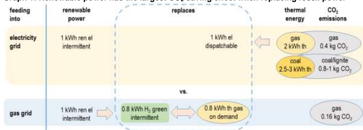
Graph 1: Renewable power has the largest CO 2 saving effect when replacing fossil power
